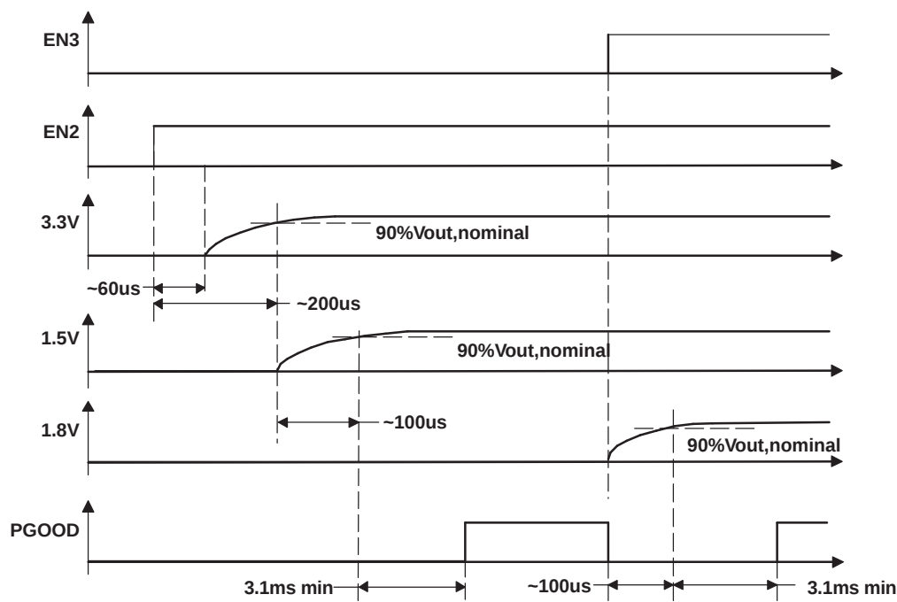
Figure 16. Timing Diagram
