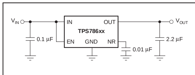
Figure 24. Typical Application Circuit
