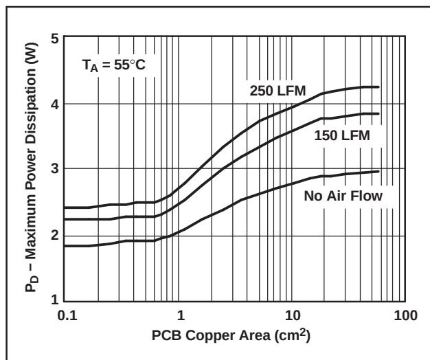
Figure 29. DPAK Maximum Power Dissipation vs PCB Copper Area
