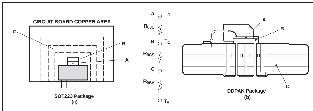
Figure 26. Thermal Resistances
