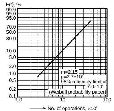
14.-(1) Contact reliability (1 mA 5 V DC resistive load) Tested sample: TQ2-12V Condition: Detection level 10 \Omega
