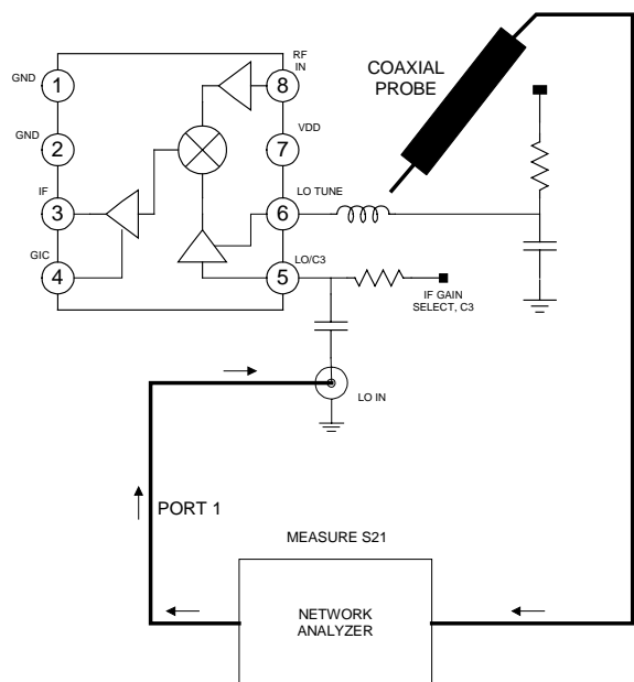
Figure 2 LO Tuning Setup
