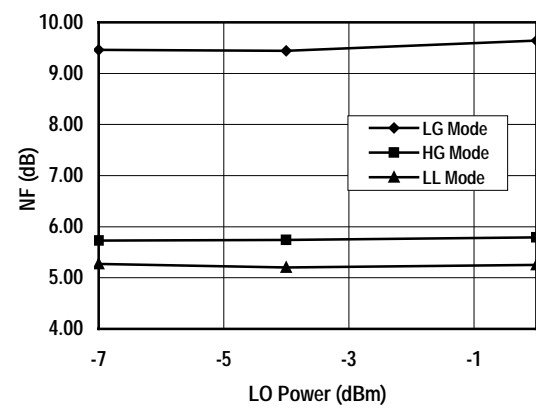
Noise Figure vs. LO Power
