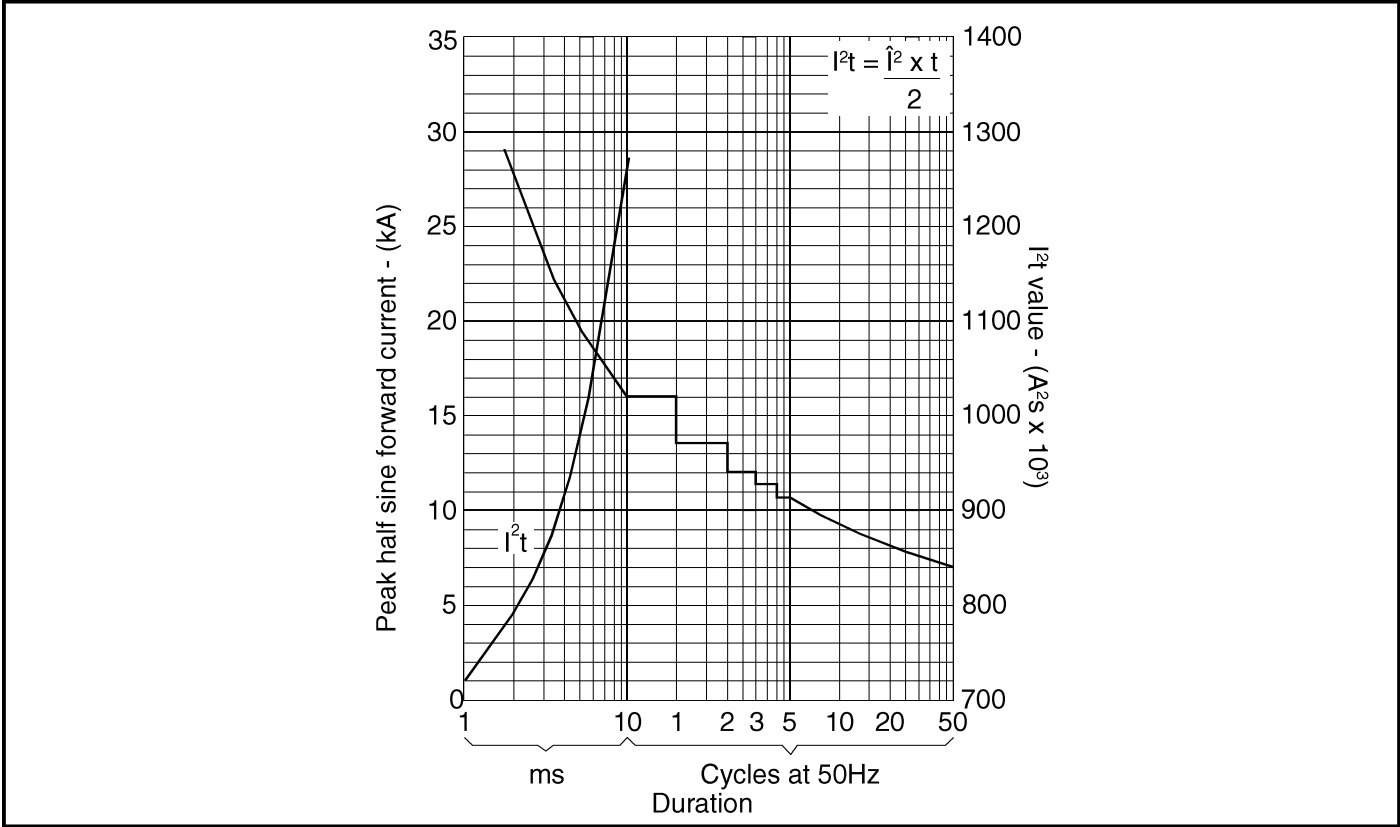
Fig. 5 Surge (non-repetitive) forward current vs time (with 50% V_{RRM} , T_{case} = 175C )
