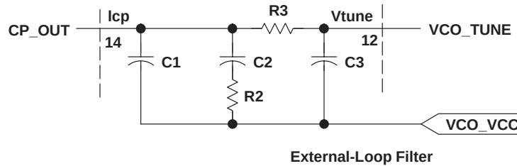
Figure 5. Third-Order Loop Filter and Transfer Function
