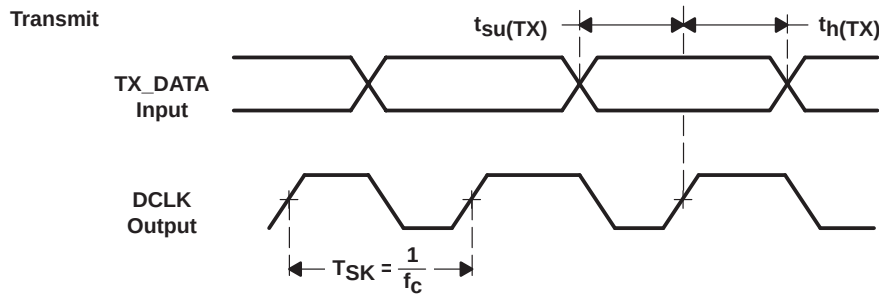
Figure 3. Timing Data for DCLK and TX_DATA
