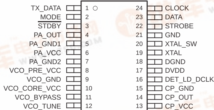
PW PACKAGE (TOP VIEW)
