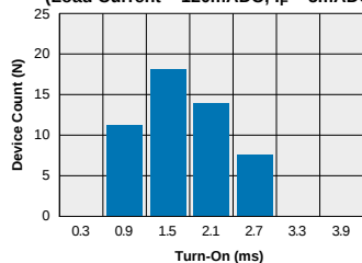
TS120 Typical Turn-On Time (N=50 Ambient Temperature = 25°C) (Load Current = 120mADC; I_F = 5\text{mA} )
