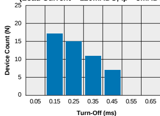
TS120 Typical Turn-Off Time (N=50 Ambient Temperature = 25°C) (Load Current = 120mADC; I_F = 5\text{mA} )
