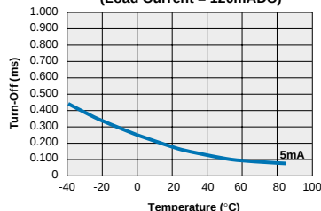
TS120 Typical Turn-Off vs. Temperature (Load Current = 120mADC)
