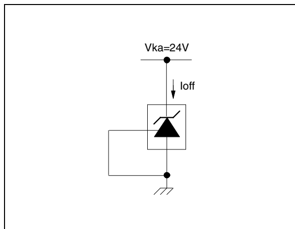
Figure 11. Test circuit for V_K > V_{REF}
