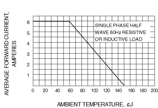
Fig. 2-FORWARD DERATING CURVE
