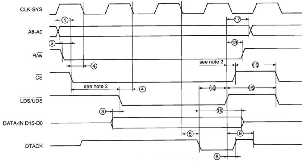
Figure 5. Write Cycle
