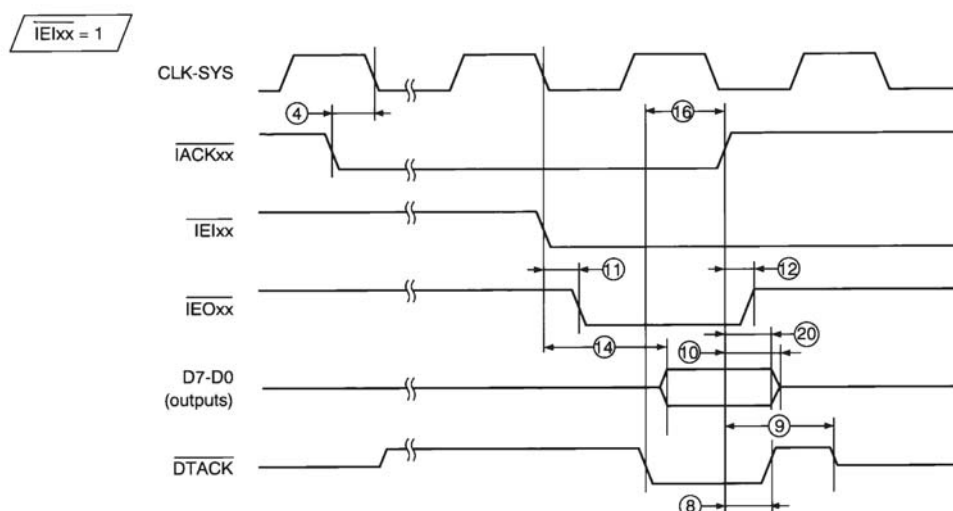
Figure 7. Interrupt Cycle ( \overline{\text{IEIxx}} = 1 )
