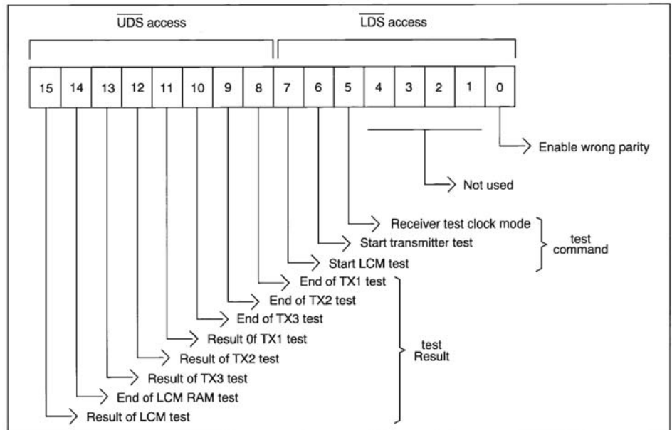
Figure 27. Self-test Register
