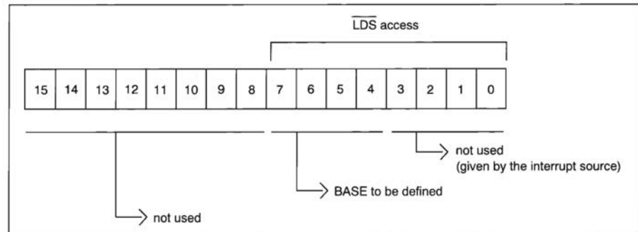
Figure 25. Base Register
