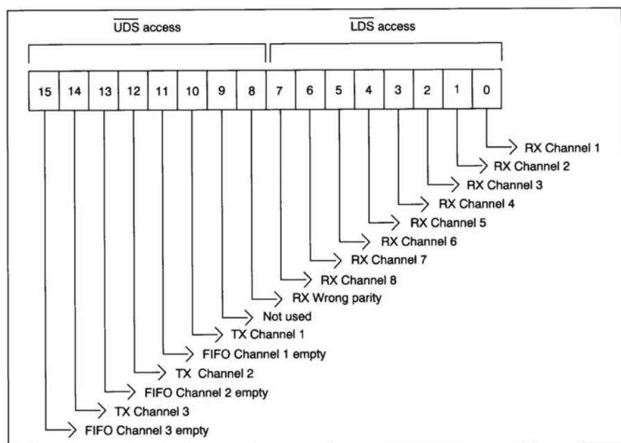
Figure 24. Mask Register
