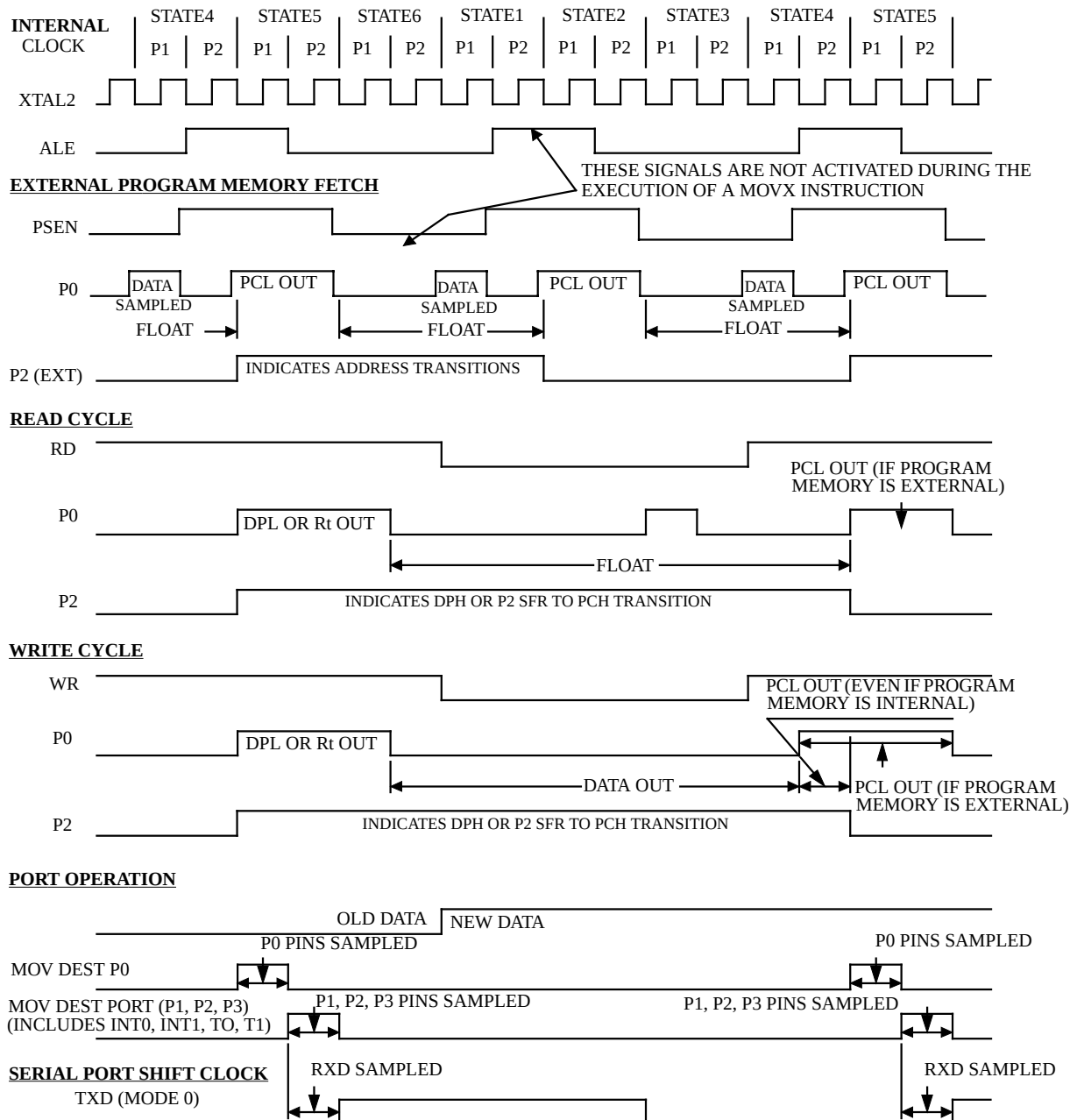
Figure 21. Clock Waveforms
