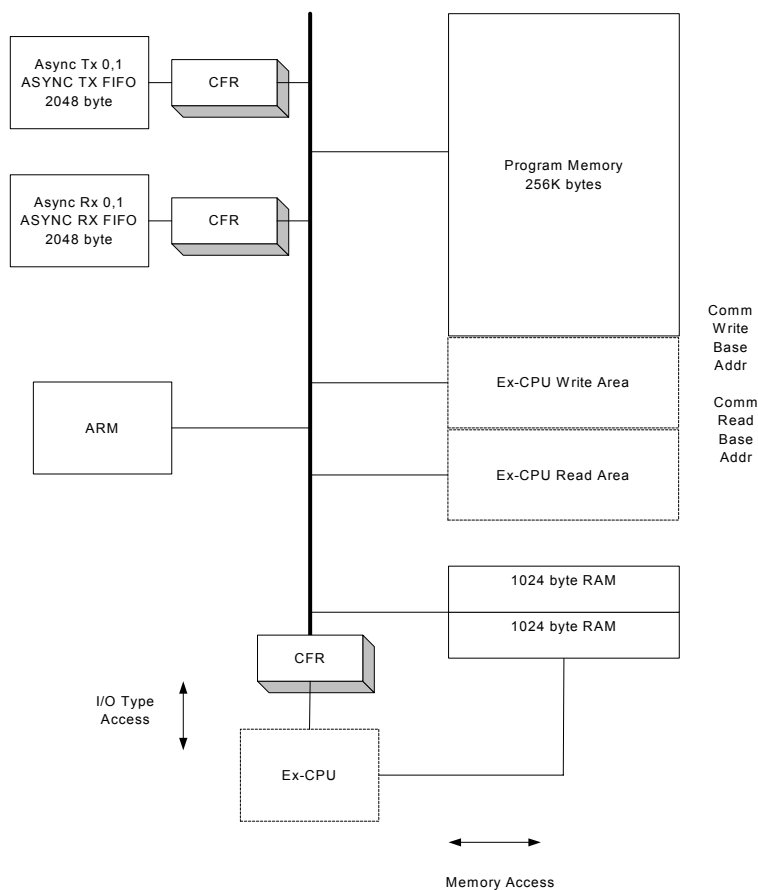
Figure 9. Ex-CPU Access
