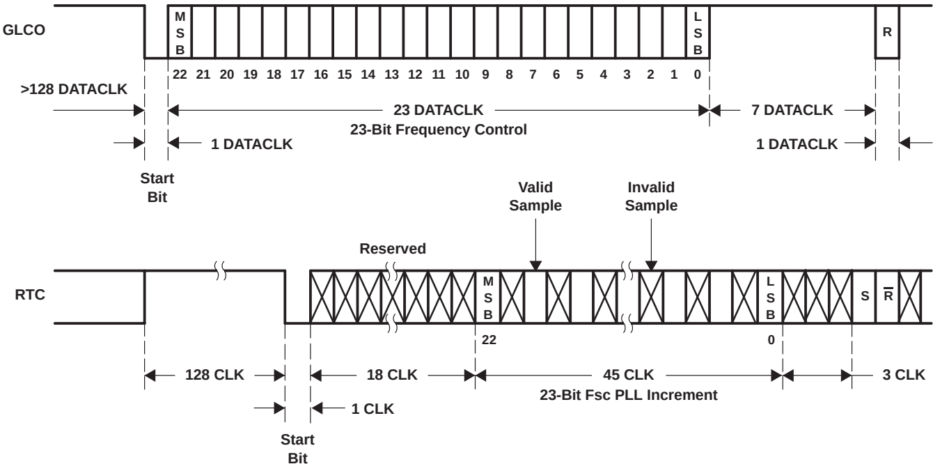
Figure 2–19. GLCO and RTC Timing
