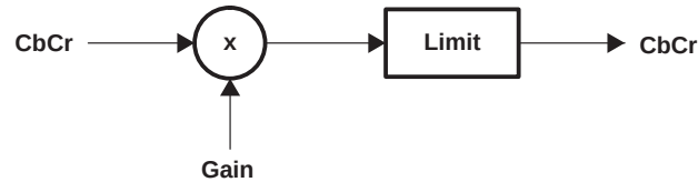
Figure 2–17. CbCr Component Gain, Offset, Limit
