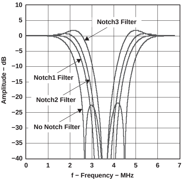
Figure 2–9. Chroma Trap Filter Frequency Response, NTSC ITU-R BT.601 Sampling
