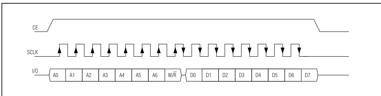
Figure 14. 3-Wire Single-Byte Read
