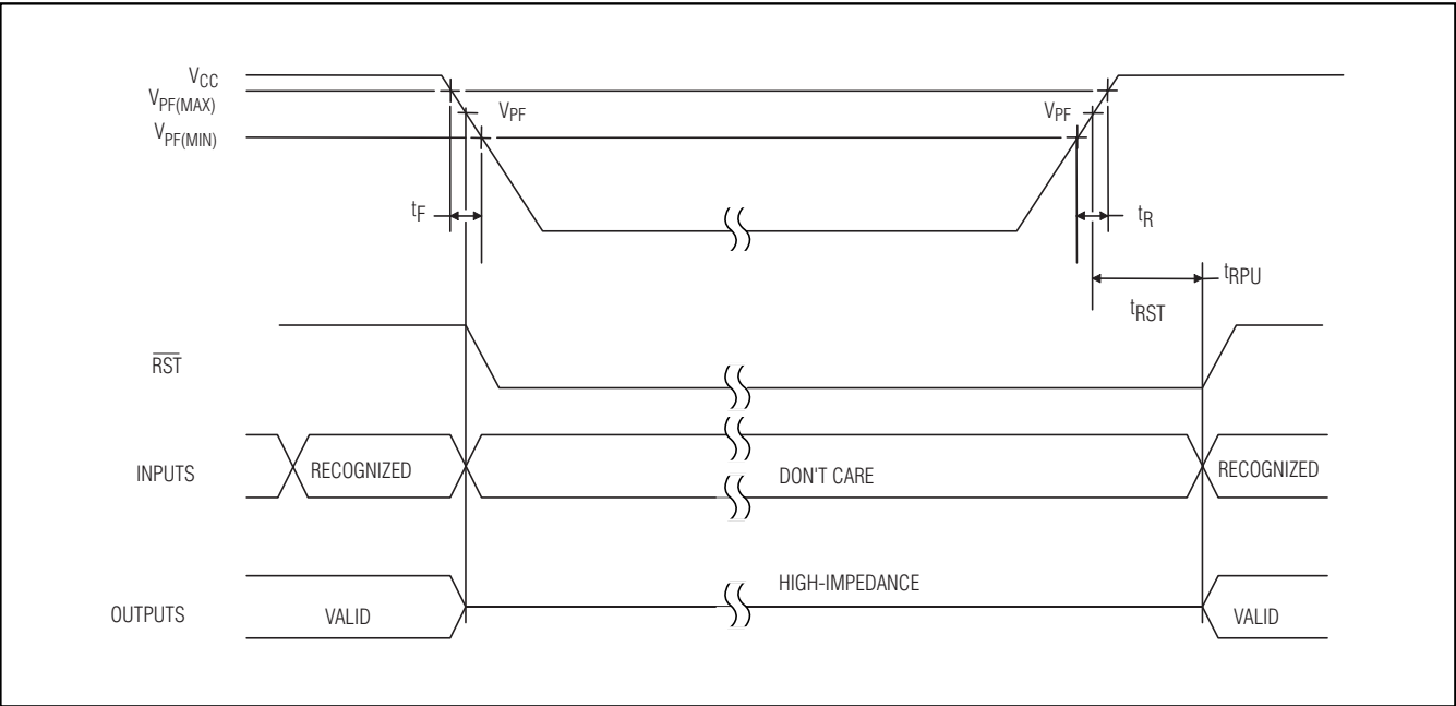
Figure 5. Power-Up/Down Timing
