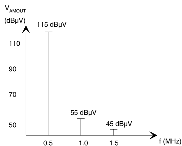
Figure 15. AM Harmonic Distortion
