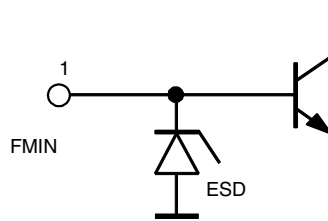
Figure 3. Internal Circuit at Pin FMIN
