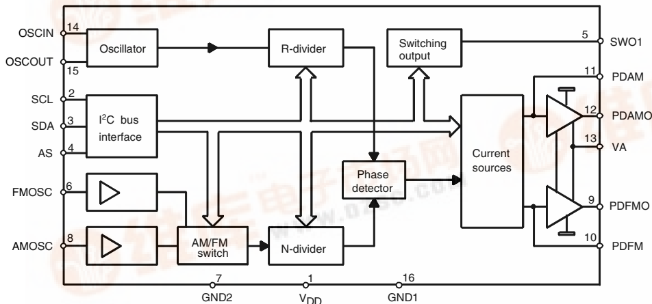
Figure 1. Block Diagram
