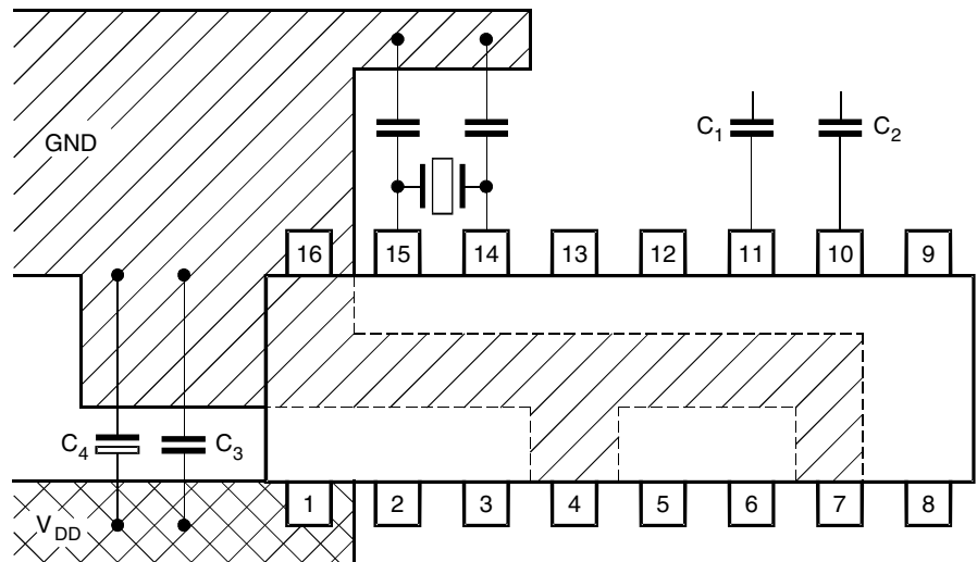
Figure 9. PCB Layout
