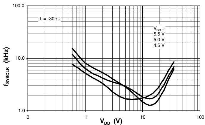
Figure 6. AM Input Sensitivity, T_{\text{amb}} = -30^{\circ}\text{C}
