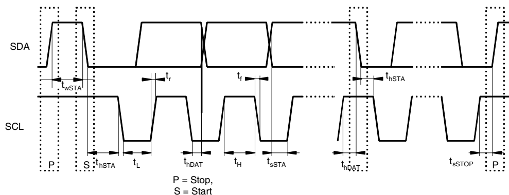
Figure 7. Bus Timing
