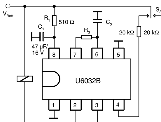
Figure 7. ON/OFF Function
