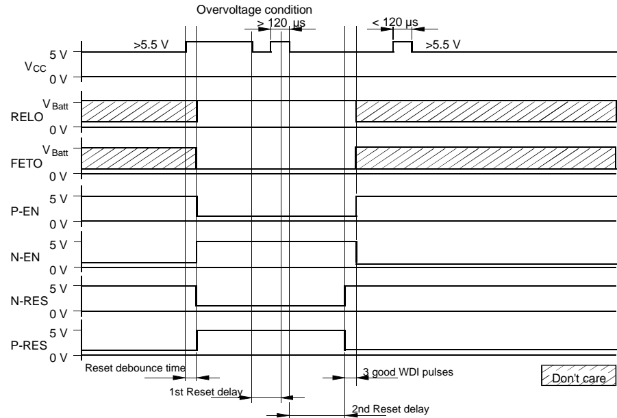
Figure 8. Overvoltage Condition
