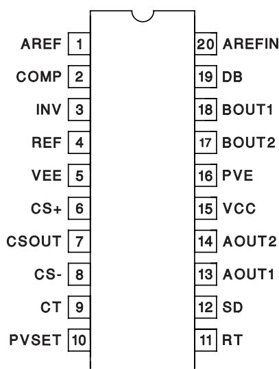
DIL-20 (Top View) N Package
