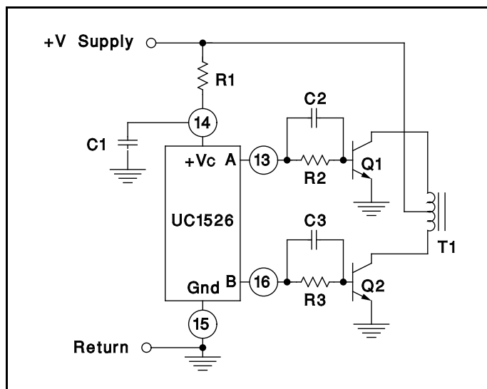
Figure 7. Push-Pull Configuration
