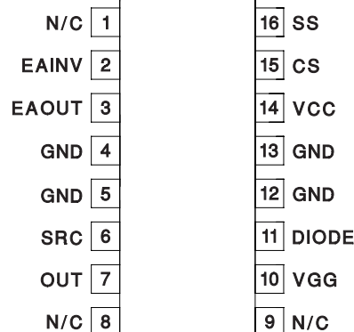
DIL-16, SOIC-16 (Top View) N or DP Packages
