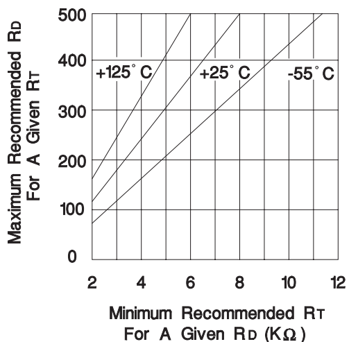
Maximum value R_D vs minimum value R_T .
