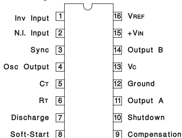
DIL-16 (TOP VIEW) J or N Package
