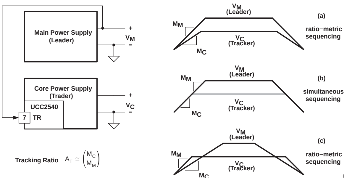
Figure 23. Ratio-Metric Tracking
