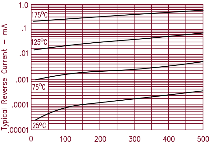
Figure 2 Typical Reverse Characteristics — Per Leg
