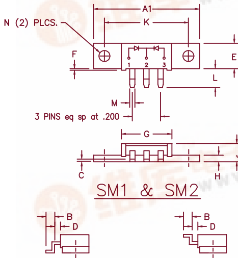
TYP. PIN CONFIGURATION FOR SM1, SM3, & SM5
