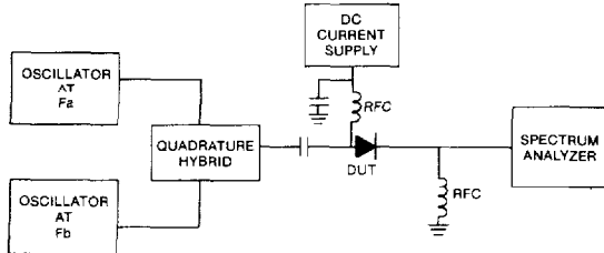
Forward Bias Distortion Test Set
