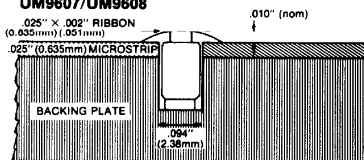
Microstrip Mount
