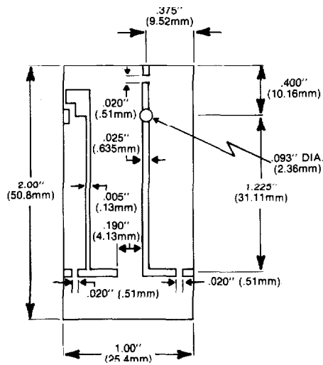
Substrate Drawing
