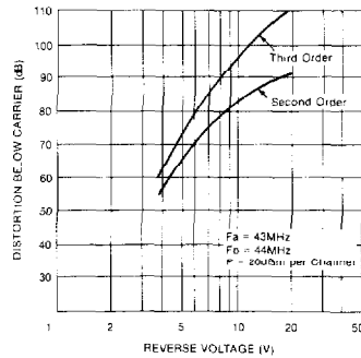
Typical Reverse Bias Intermodulation Distortion
