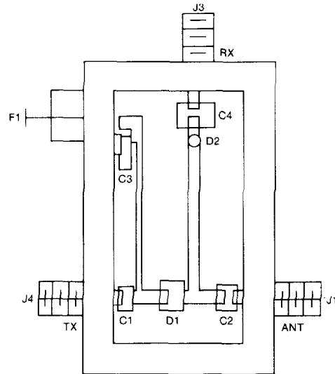
Assembly Drawing
