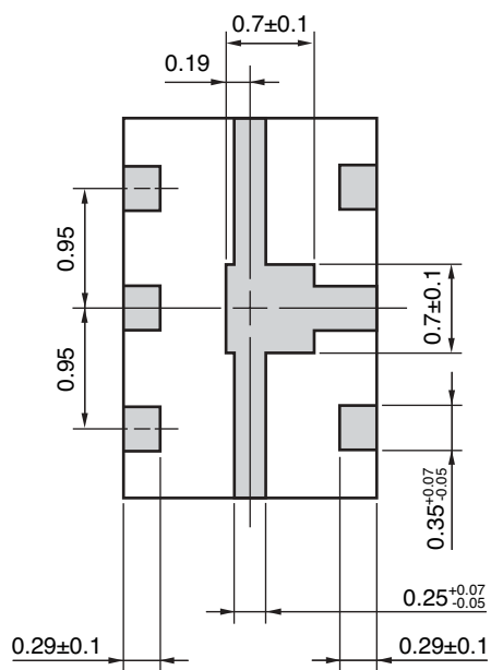
(Bottom View)
