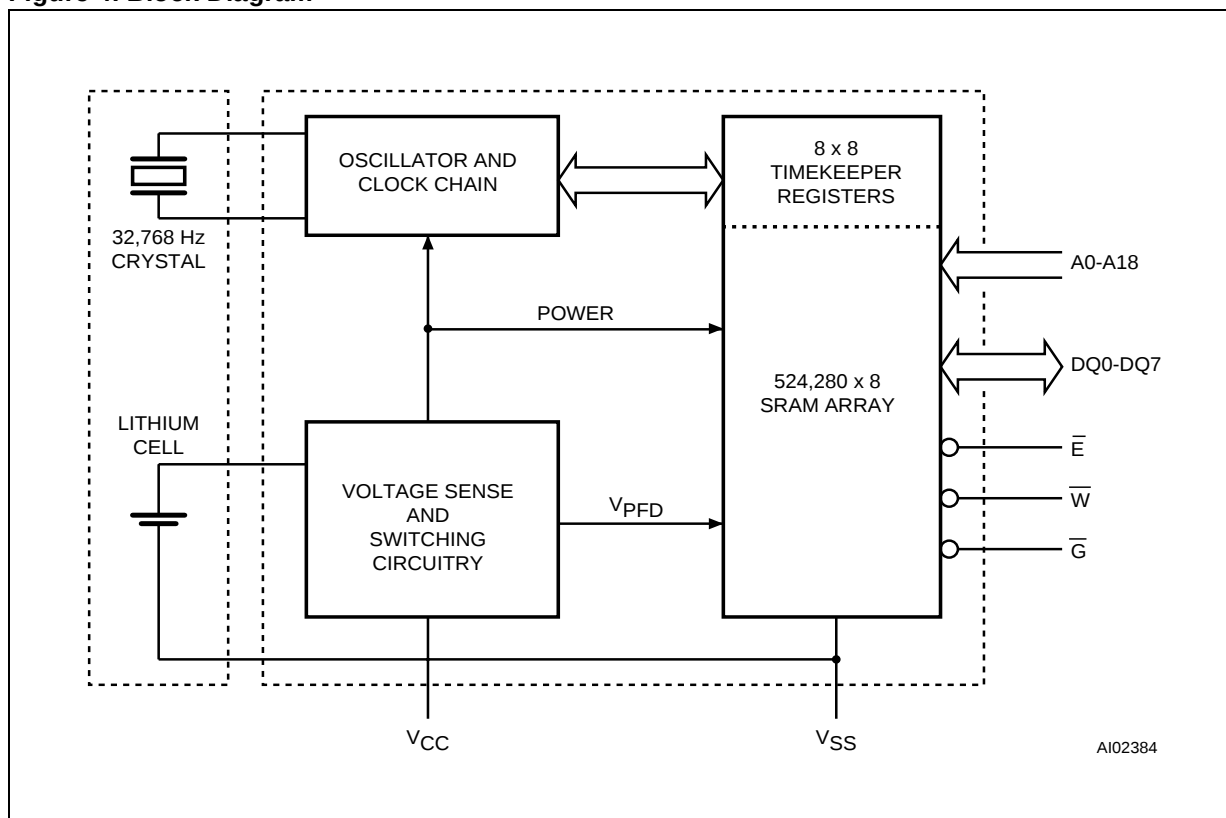
Figure 4. Block Diagram
