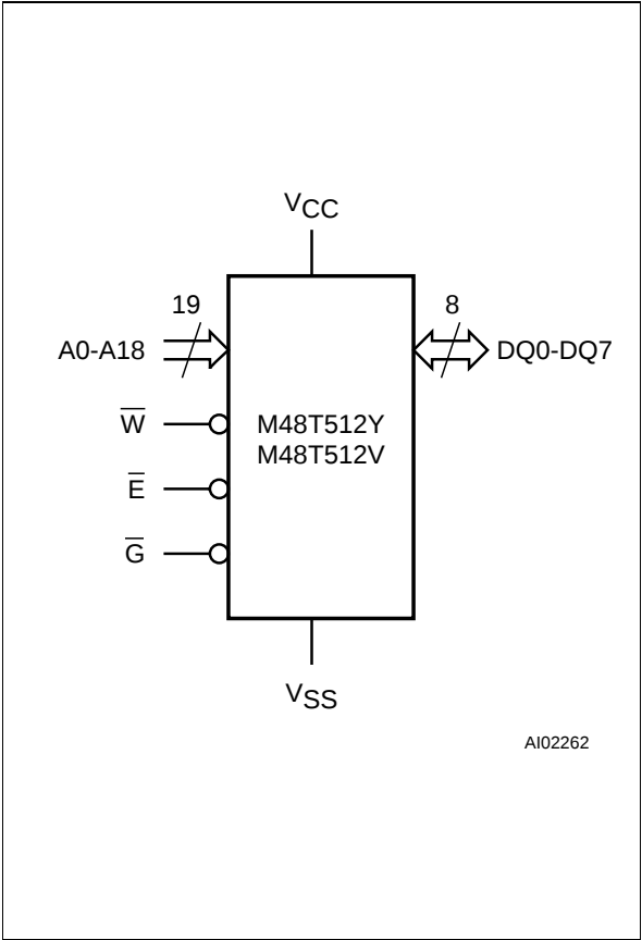
Figure 1. Logic Diagram
