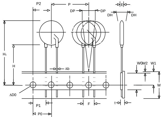
In Line Leads "L3"
