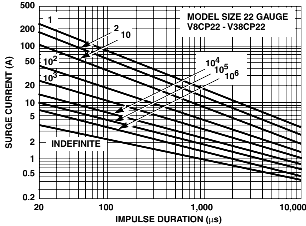
FIGURE 15. SURGE CURRENT RATING CURVES FOR V8CP22 - V38CP22
