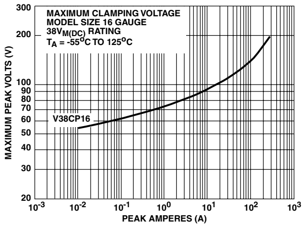
FIGURE 3. CLAMPING VOLTAGE FOR V38CP16
