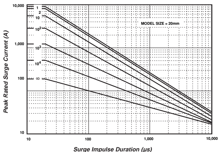
Figure 9. Repetitive Surge Capability for 20mm Parts (V130LA20C(P)-V680LA100C(P))
