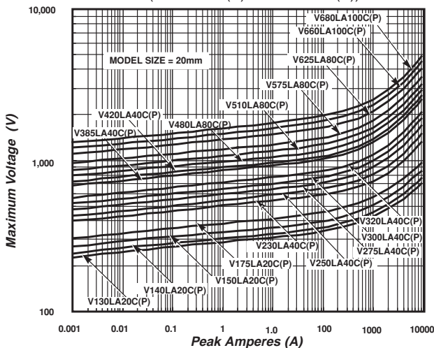
Figure 5. Maximum Clamping Voltage for 20mm Parts (V130LA20C(P) -V680LA100C(P))
