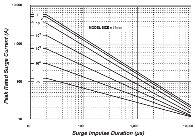
Figure 8. Repetitive Surge Capability for 14mm Parts (V130LA10C(P)-V420LA20C(P))
