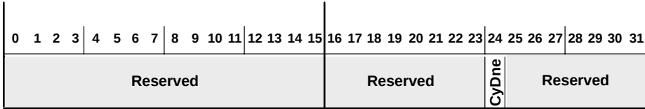
Figure 4–20. CycleMark Format
