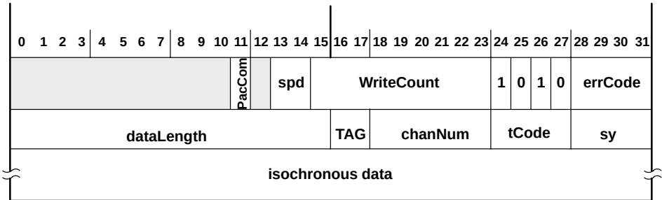
Figure 4–18. Isochronous-Receive Format
