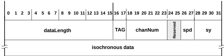
Figure 4–17. Isochronous-Transmit Format
