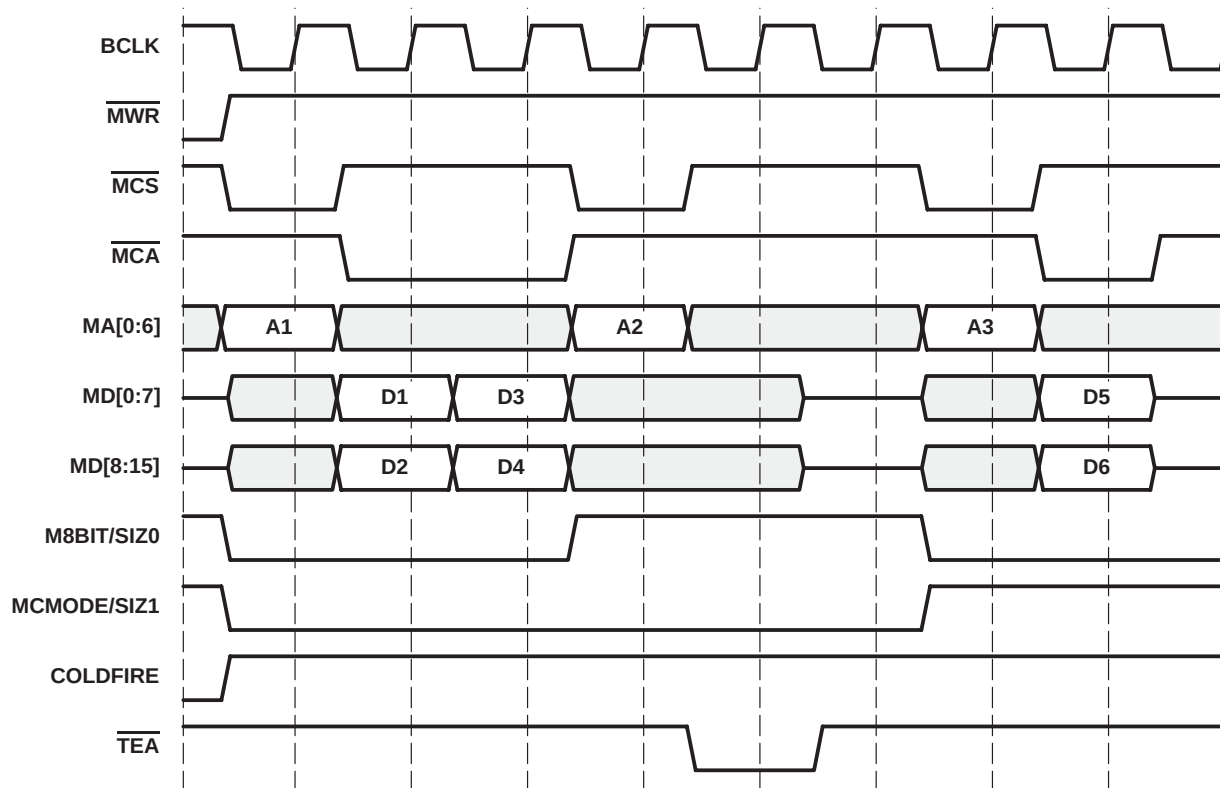
Figure 3–13. ColdFire Read
