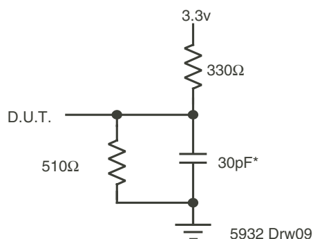
Figure 7. Output Load
