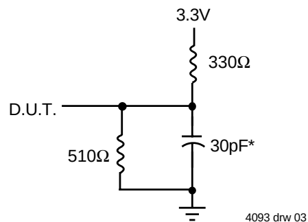
Figure 1. Output Load
