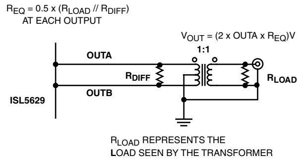
FIGURE 6. OUTPUT LOADING FOR DATASHEET MEASUREMENTS
