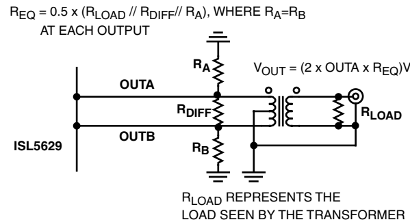
FIGURE 7. ALTERNATIVE OUTPUT LOADING
