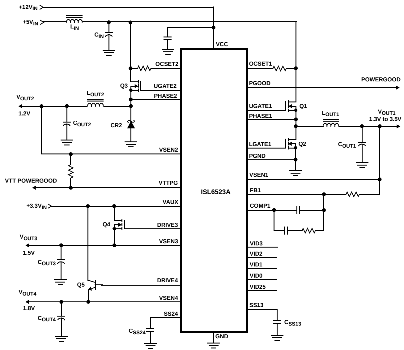
FIGURE 3. TYPICAL APPLICATION
