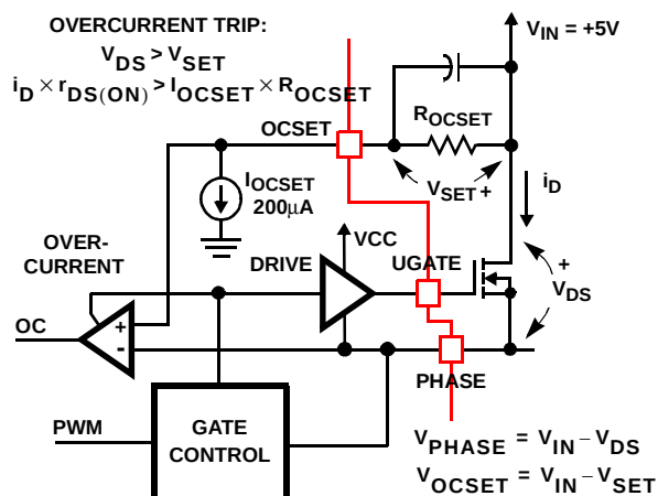
FIGURE 8. OVERCURRENT DETECTION
