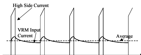
FIGURE 43. INPUT CAPACITOR FILTERS OUT THE INPUT CURRENT REQUIREMENT OF THE VRM AND LIMITS THE SLEW RATE OF THE INPUT CURRENT
