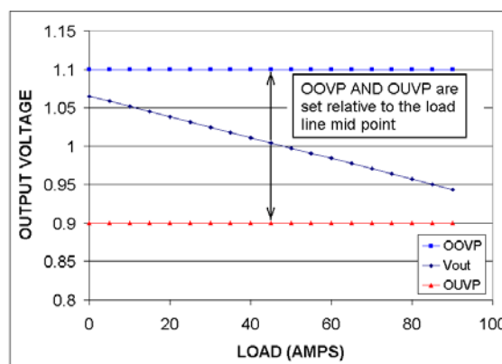
FIGURE 29. OOVP OUVP TRIP LEVELS AND LOAD LINE
