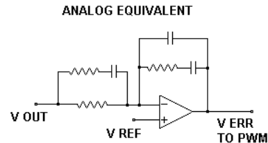
FIGURE 14. TYPICAL ANALOG ERROR AMPLIFIER AND COMPENSATION
