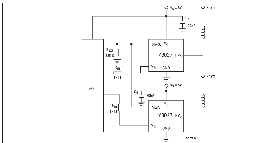
FIGURE 1: Application circuit
