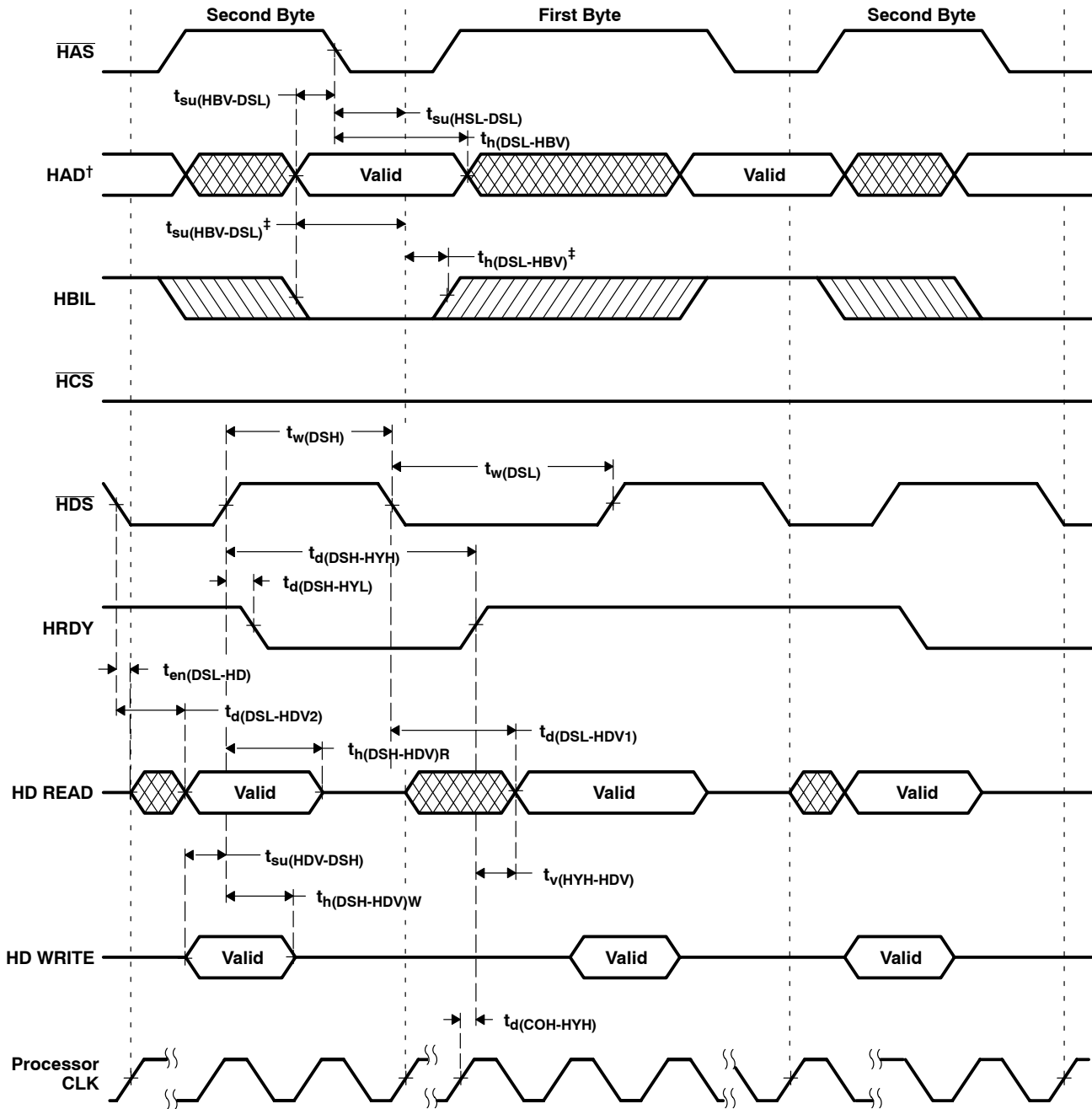
Figure 5–28. Using HDS to Control Accesses ( \overline{HCS} Always Low)
