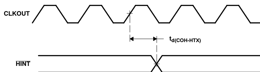
Figure 5-30. HINT Timing
