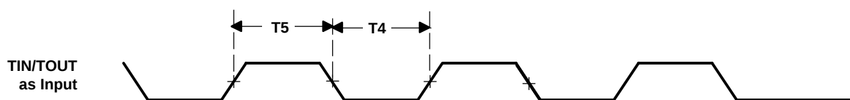
Figure 5–22. TIN/TOUT Timings When Configured as Inputs
