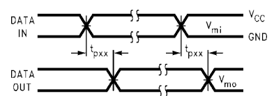
FIGURE 6. Waveform for Inverting and Non-Inverting Functions
