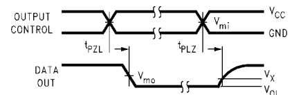
FIGURE 8. 3-STATE Output Low Enable and Disable Times for Low Voltage Logic
