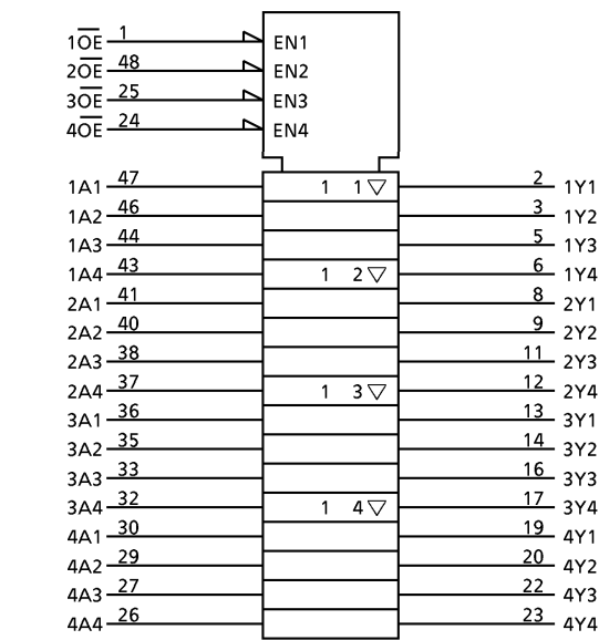
IEC LOGIC SYMBOL
