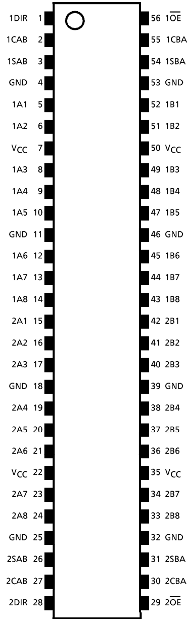
(TOP VIEW)
