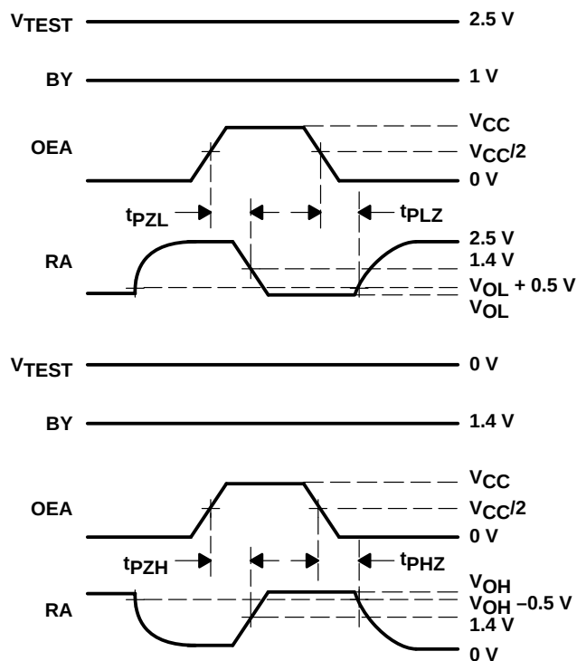
Figure 20. B-to-A Enable/Disable Time Test Circuit and Definitions
