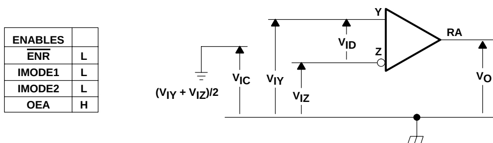
Figure 16. Voltage Definitions
