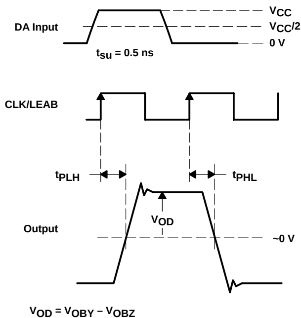
Figure 22. A-to-B Flip-Flop Mode Timing Circuit
