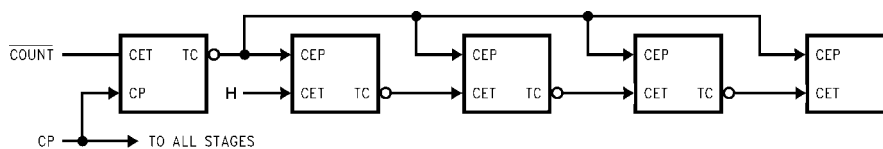
FIGURE 2. Multistage Counter with Lookahead Carry
