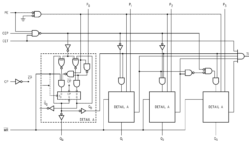
Block Diagram
