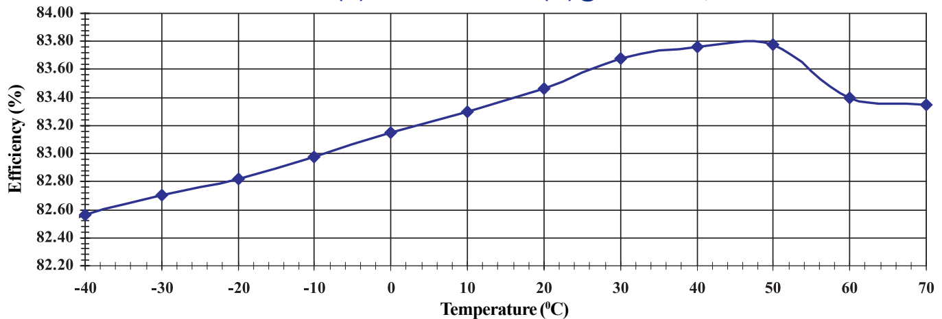
EFFICIENCY (%) vs. AMBIENT TEMP. ( ^{\circ}\text{C} ) @ V_{in} = 48\text{Vdc} ; I_o = 30\text{A}
