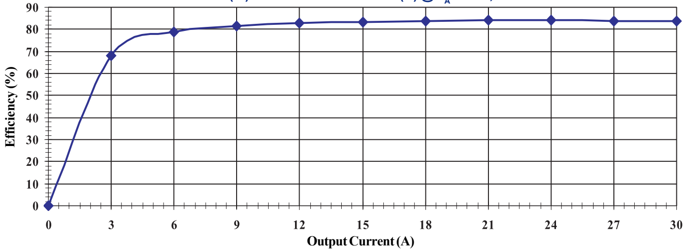
EFFICIENCY (%) vs. OUTPUT CURRENT (A) @ T_A +25^{\circ}\text{C} ; V_{in} = 48\text{Vdc}
