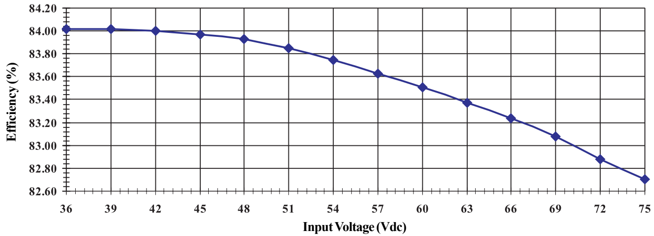
EFFICIENCY (%) vs. INPUT VOLTAGE @ T_A +25^{\circ}\text{C} ; I_o = 30\text{A}
