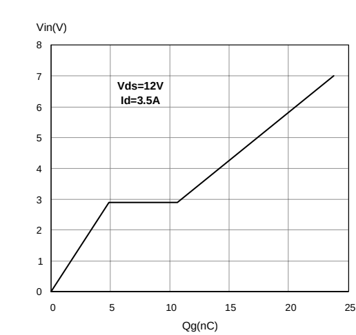
Input Voltage Vs. Input Charge
