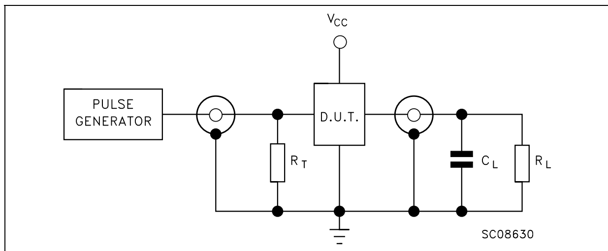
Figure 5: Test Circuit
