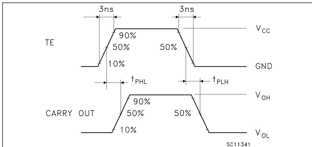
Figure 10: Waveform - Propagation Delays Cascade Mode ( f=1\text{MHz} ; 50% duty cycle)
