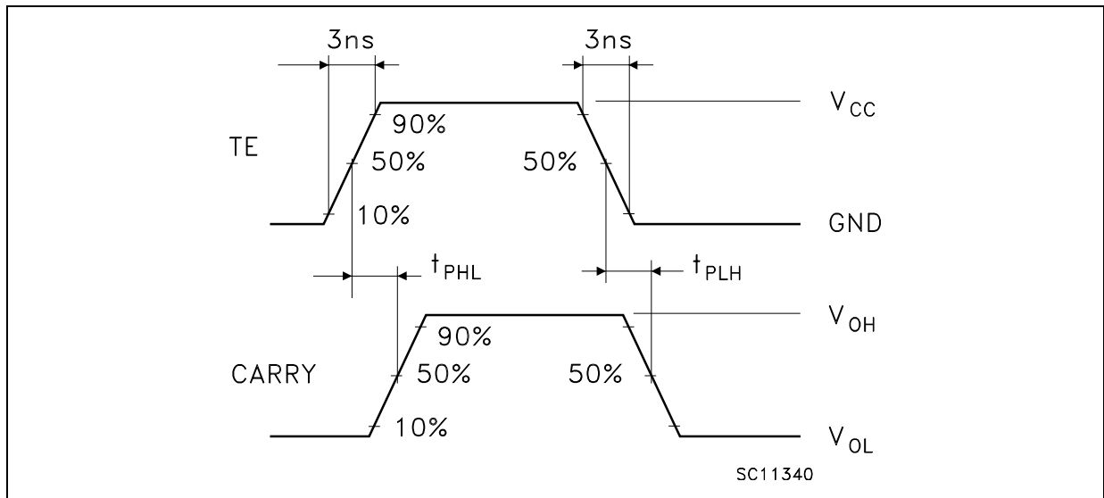
WAVEFORM 5: PROPAGATION DELAYS CASCADE MODE ( f=1\text{MHz} ; 50% duty cycle)
