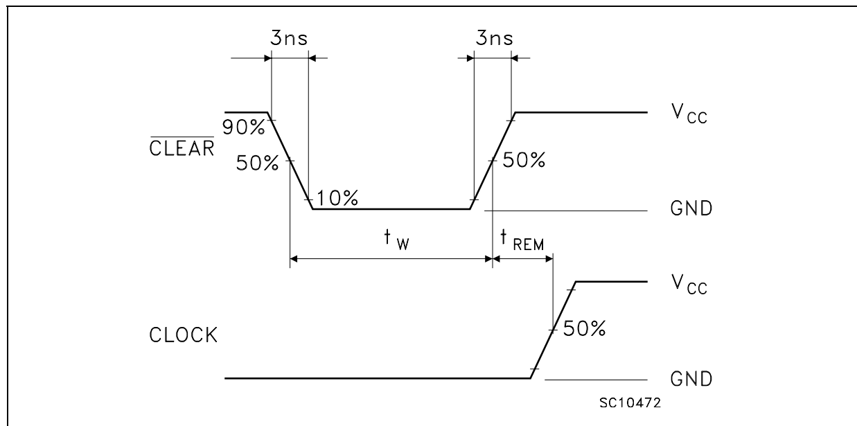
Figure 8: Waveform - Recovery Time ( f=1\text{MHz} ; 50% duty cycle)
